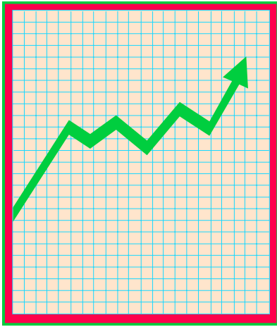
Figure 1. Database contexts
