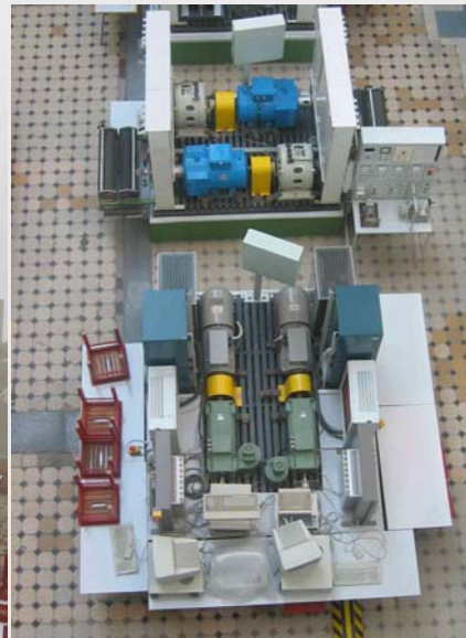
Universal lab stand electric drives
