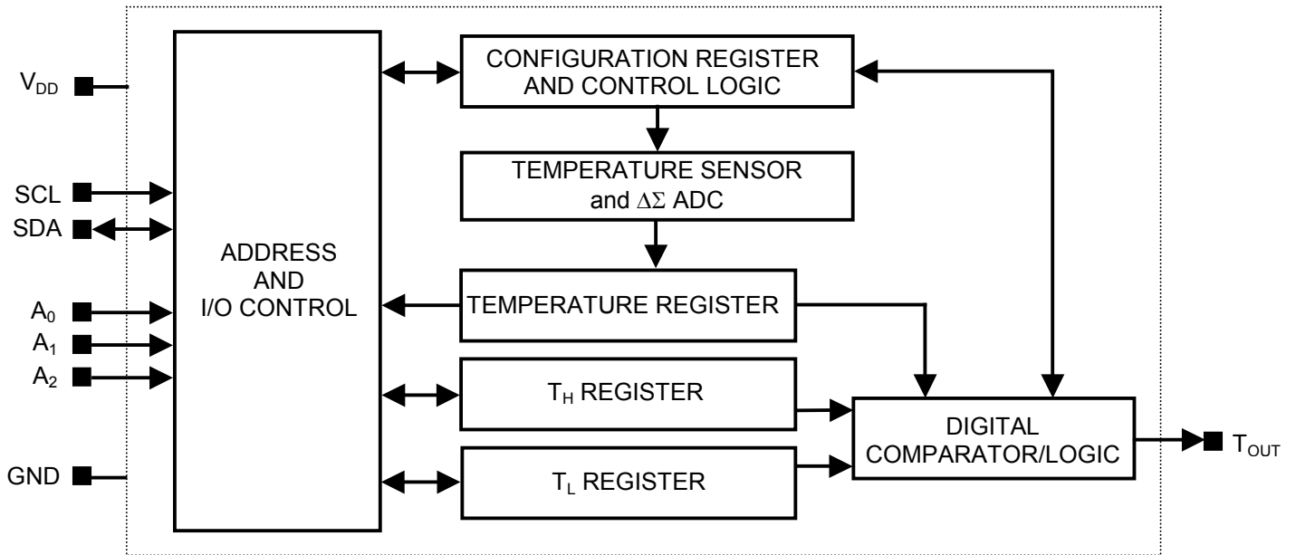
Figure 1. FUNCTIONAL DIAGRAM
